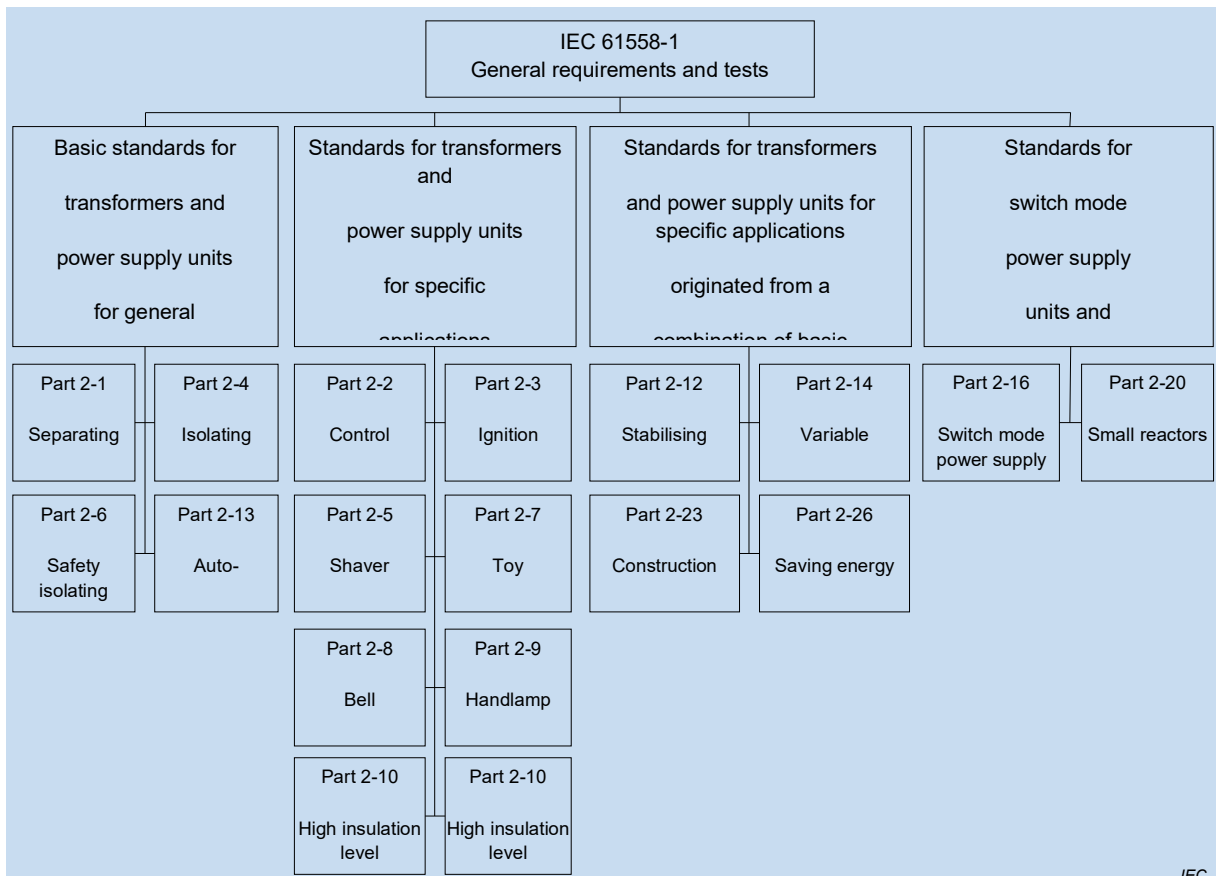
Figure 1 – IEC 61558 principle
